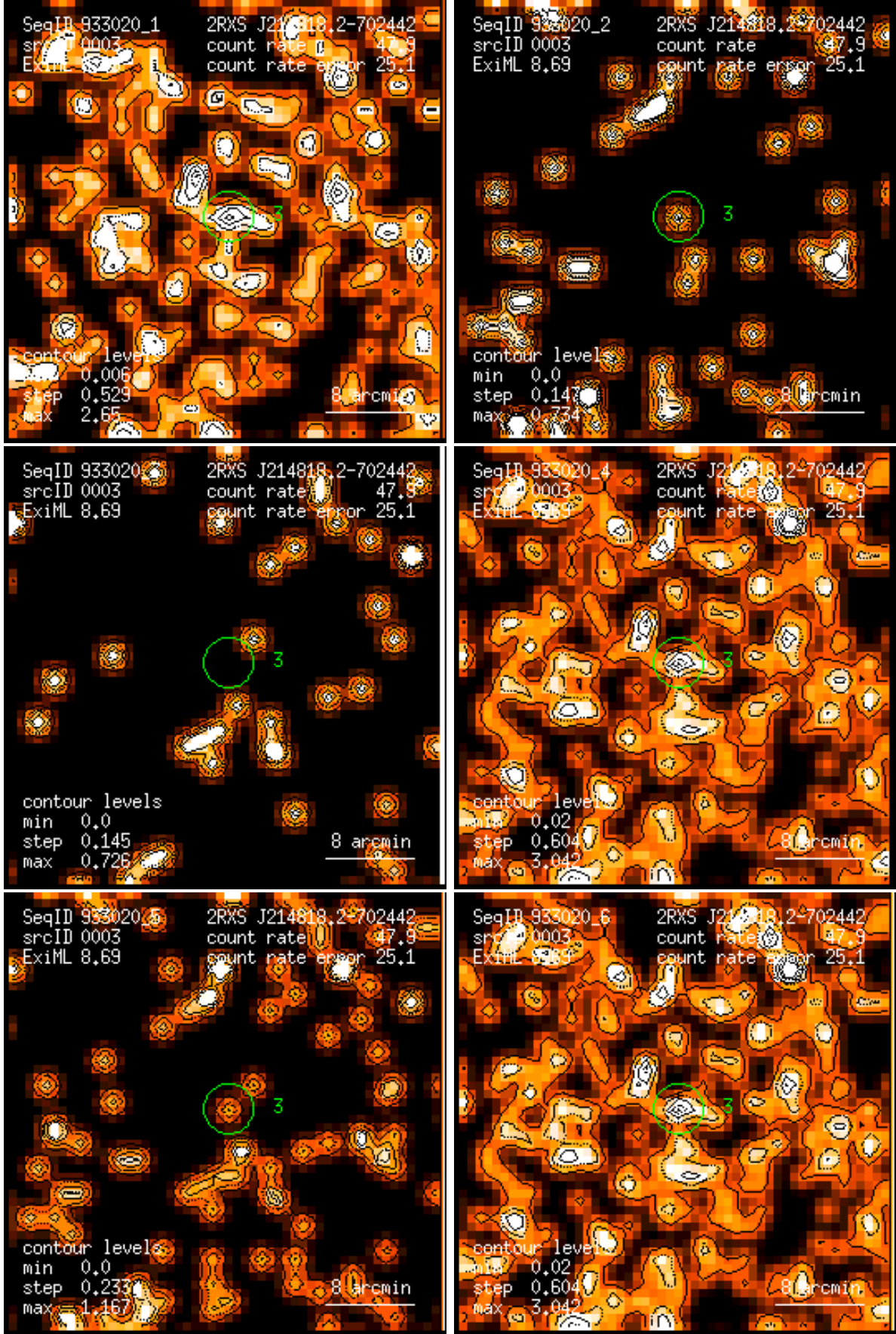
Figure 3: RASS 933020: detection 0003: band rate images, Gaussian filter: (1) PSPC channels 11 – 41, (2) 52 – 90, (3) 91 – 201, (4) 11 – 235, (5) 52 – 201, (6) 11 – 201. Broad band rates in counts/ks. Band rate contour levels in counts/ks/arcmin 2 .
