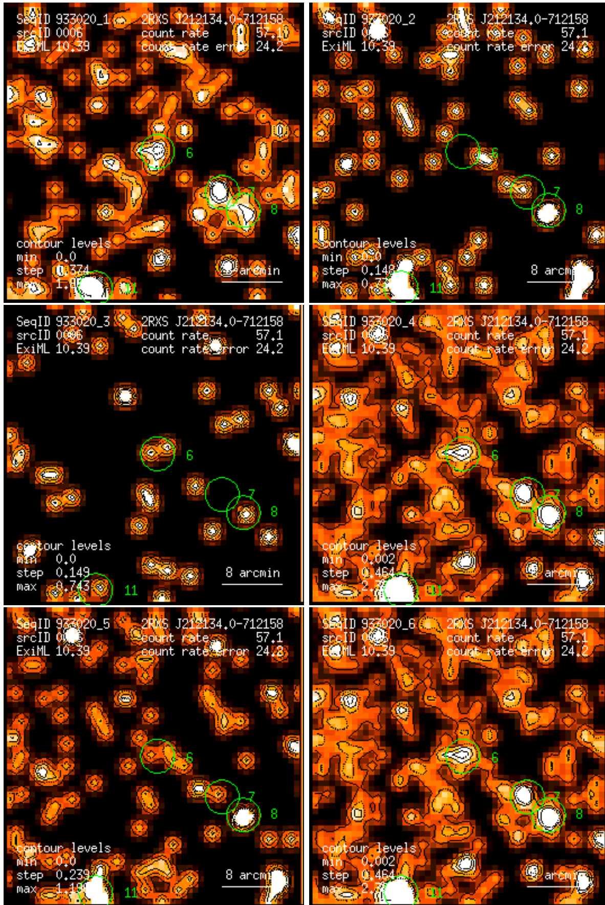
Figure 6: RASS 933020: detection 0006: band rate images, Gaussian filter: (1) PSPC channels 11 – 41, (2) 52 – 90, (3) 91 – 201, (4) 11 – 235, (5) 52 – 201, (6) 11 – 201. Broad band rates in counts/ks. Band rate contour levels in counts/ks/arcmin 2 .
