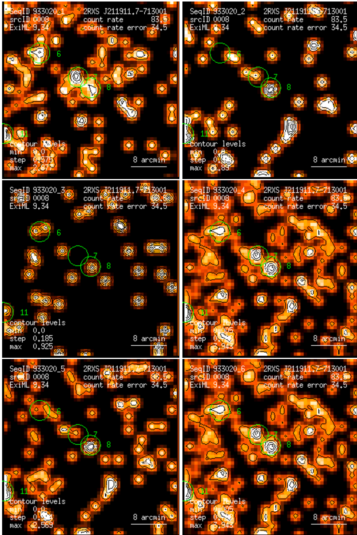
Figure 8: RASS 933020: detection 0008: band rate images, Gaussian filter: (1) PSPC channels 11 – 41, (2) 52 – 90, (3) 91 – 201, (4) 11 – 235, (5) 52 – 201, (6) 11 – 201. Broad band rates in counts/ks. Band rate contour levels in counts/ks/arcmin 2 .
