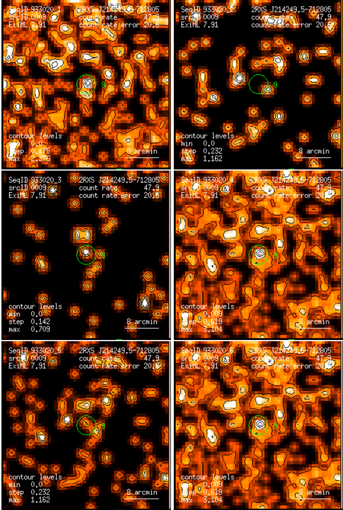
Figure 9: RASS 933020: detection 0009: band rate images, Gaussian filter: (1) PSPC channels 11 – 41, (2) 52 – 90, (3) 91 – 201, (4) 11 – 235, (5) 52 – 201, (6) 11 – 201. Broad band rates in counts/ks. Band rate contour levels in counts/ks/arcmin 2 .
