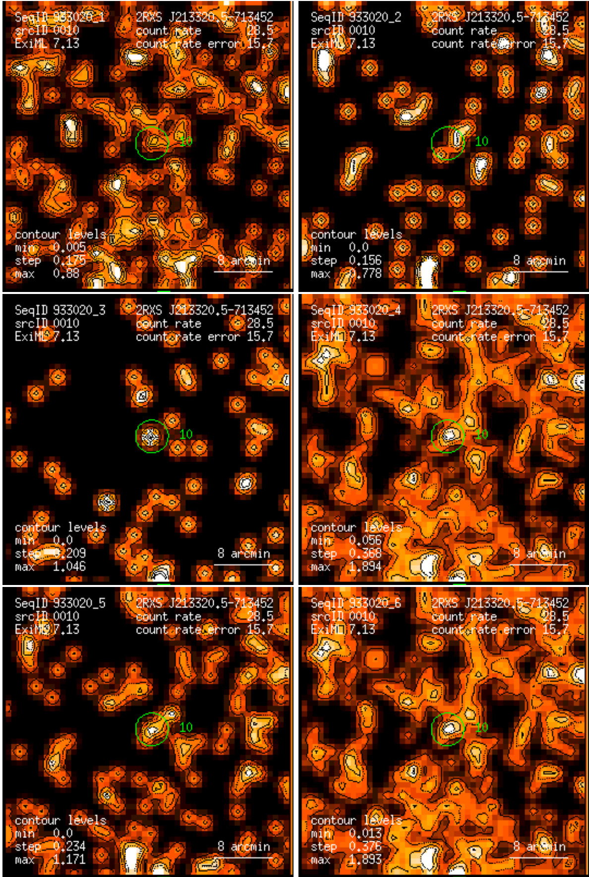
Figure 10: RASS 933020: detection 0010: band rate images, Gaussian filter: (1) PSPC channels 11 – 41, (2) 52 – 90, (3) 91 – 201, (4) 11 – 235, (5) 52 – 201, (6) 11 – 201. Broad band rates in counts/ks. Band rate contour levels in counts/ks/arcmin 2 .
