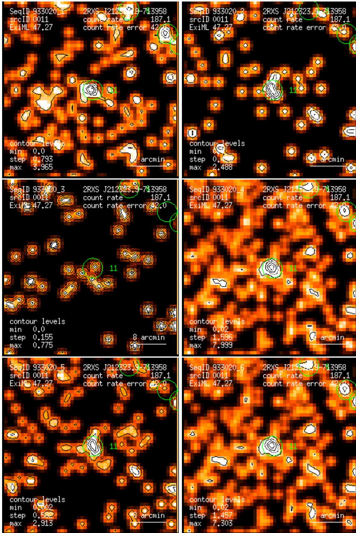
Figure 11: RASS 933020: detection 0011: band rate images, Gaussian filter: (1) PSPC channels 11 – 41, (2) 52 – 90, (3) 91 – 201, (4) 11 – 235, (5) 52 – 201, (6) 11 – 201. Broad band rates in counts/ks. Band rate contour levels in counts/ks/arcmin 2 .
