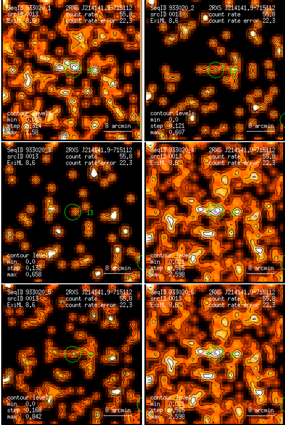
Figure 13: RASS 933020: detection 0013: band rate images, Gaussian filter: (1) PSPC channels 11 – 41, (2) 52 – 90, (3) 91 – 201, (4) 11 – 235, (5) 52 – 201, (6) 11 – 201. Broad band rates in counts/ks. Band rate contour levels in counts/ks/arcmin 2 .
