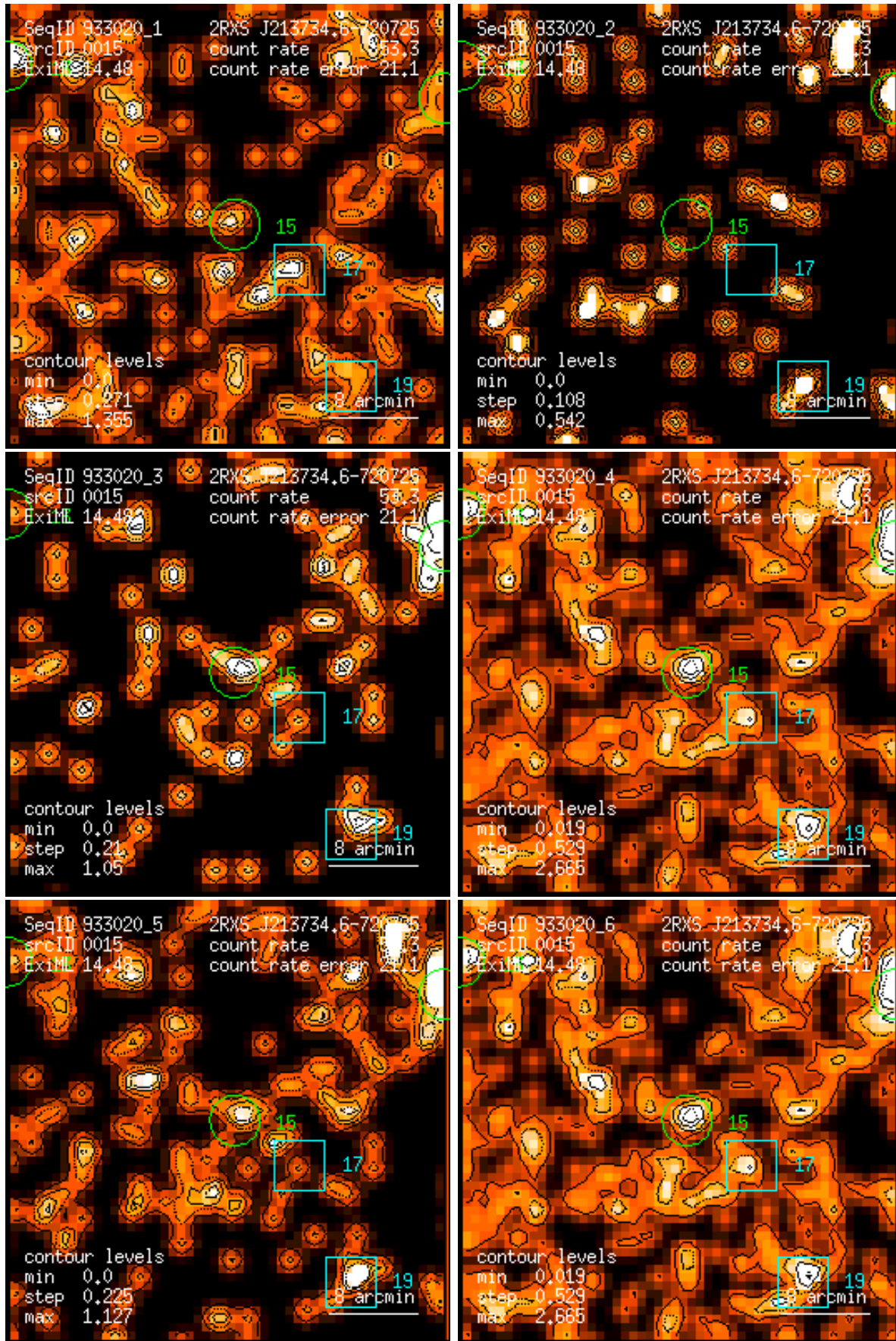
Figure 15: RASS 933020: detection 0015: band rate images, Gaussian filter: (1) PSPC channels 11 – 41, (2) 52 – 90, (3) 91 – 201, (4) 11 – 235, (5) 52 – 201, (6) 11 – 201. Broad band rates in counts/ks. Band rate contour levels in counts/ks/arcmin 2 .
