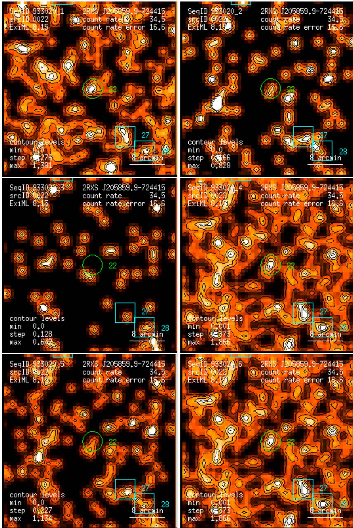
Figure 22: RASS 933020: detection 0022: band rate images, Gaussian filter: (1) PSPC channels 11 – 41, (2) 52 – 90, (3) 91 – 201, (4) 11 – 235, (5) 52 – 201, (6) 11 – 201. Broad band rates in counts/ks. Band rate contour levels in counts/ks/arcmin 2 .
