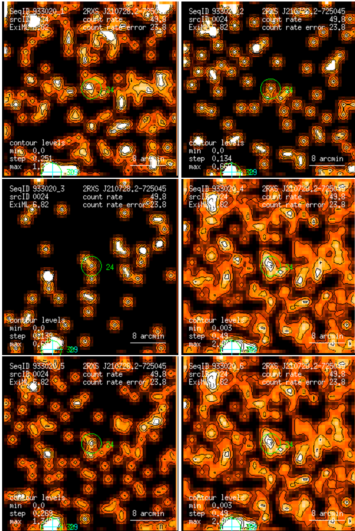
Figure 24: RASS 933020: detection 0024: band rate images, Gaussian filter: (1) PSPC channels 11 – 41, (2) 52 – 90, (3) 91 – 201, (4) 11 – 235, (5) 52 – 201, (6) 11 – 201. Broad band rates in counts/ks. Band rate contour levels in counts/ks/arcmin 2 .
