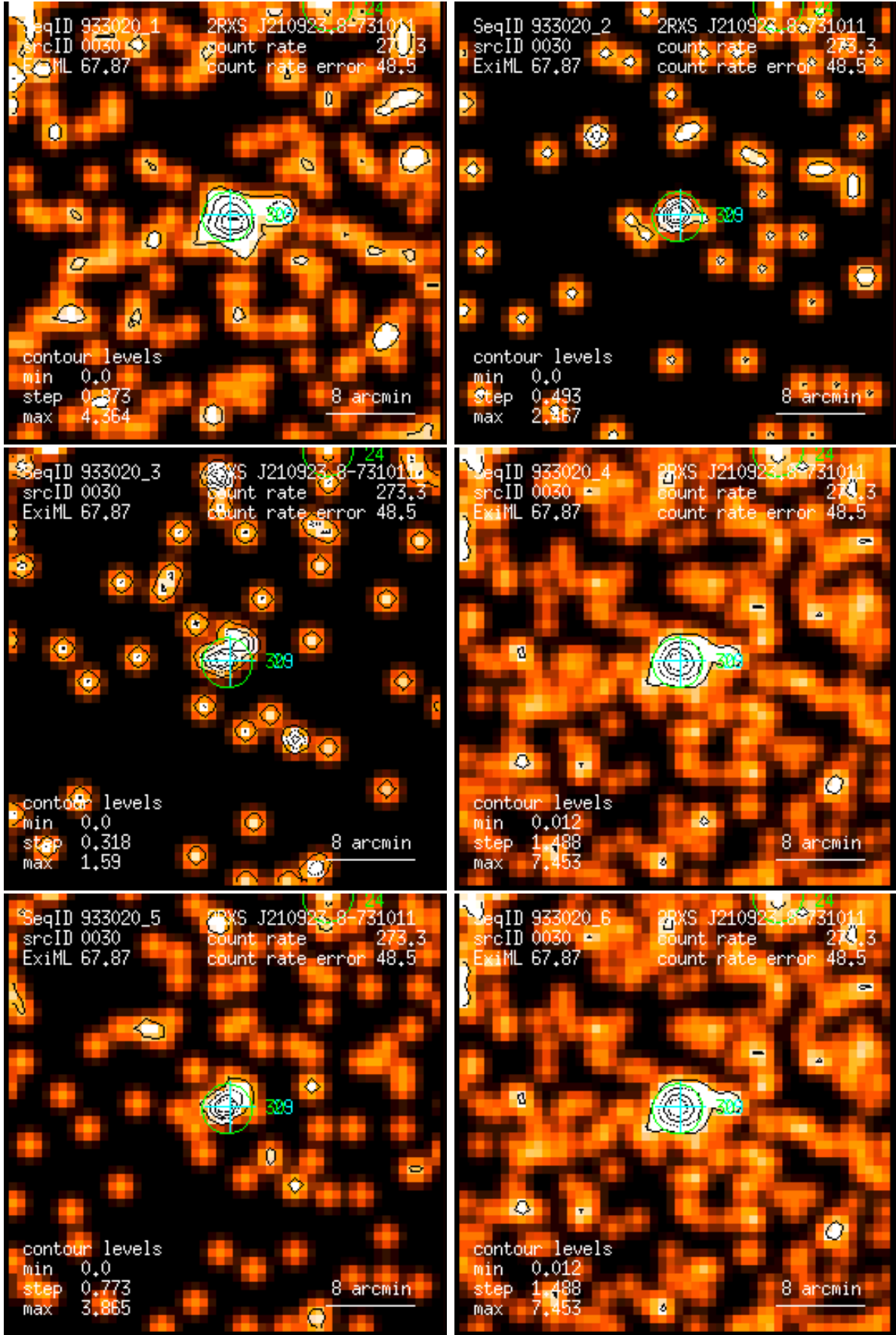
Figure 30: RASS 933020: detection 0030: band rate images, Gaussian filter: (1) PSPC channels 11 – 41, (2) 52 – 90, (3) 91 – 201, (4) 11 – 235, (5) 52 – 201, (6) 11 – 201. Broad band rates in counts/ks. Band rate contour levels in counts/ks/arcmin 2 .
