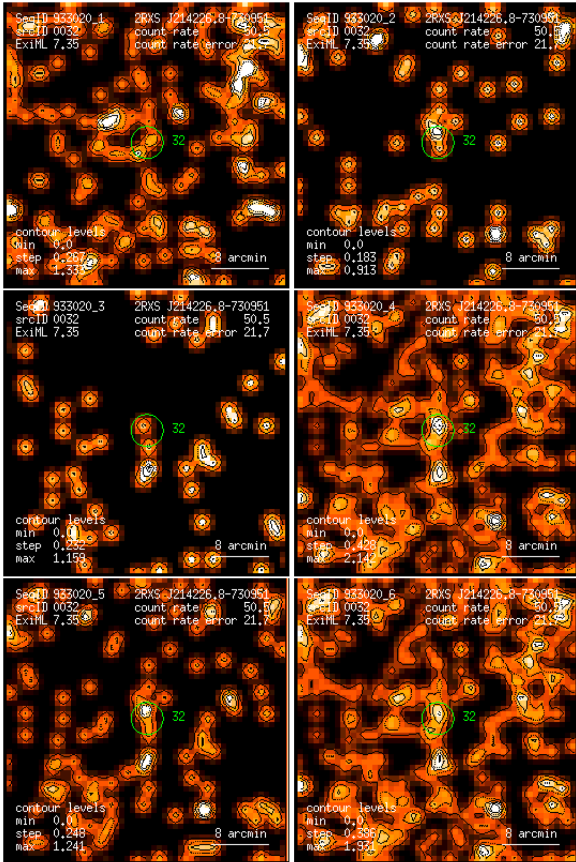
Figure 32: RASS 933020: detection 0032: band rate images, Gaussian filter: (1) PSPC channels 11 – 41, (2) 52 – 90, (3) 91 – 201, (4) 11 – 235, (5) 52 – 201, (6) 11 – 201. Broad band rates in counts/ks. Band rate contour levels in counts/ks/arcmin 2 .
