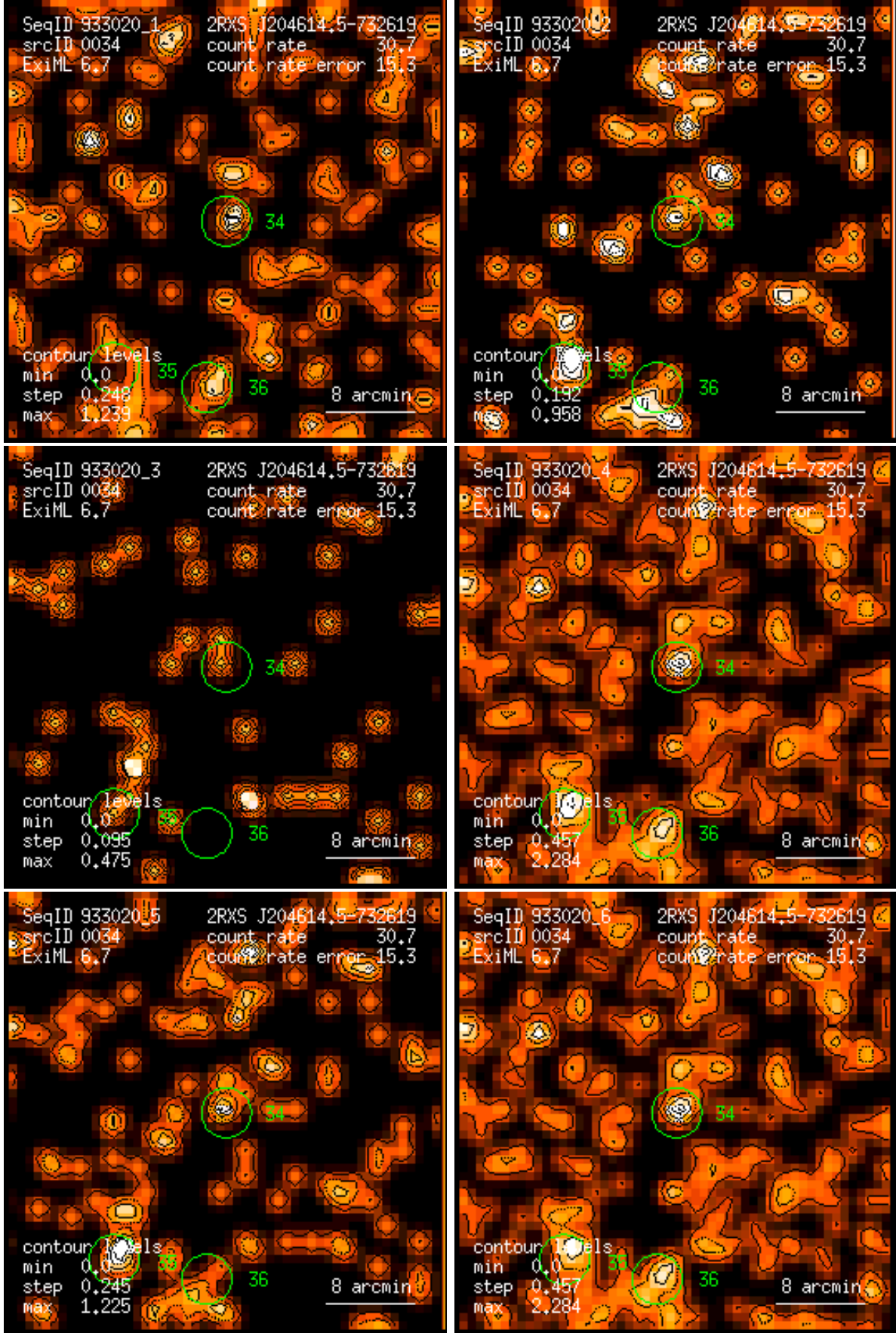
Figure 34: RASS 933020: detection 0034: band rate images, Gaussian filter: (1) PSPC channels 11 – 41, (2) 52 – 90, (3) 91 – 201, (4) 11 – 235, (5) 52 – 201, (6) 11 – 201. Broad band rates in counts/ks. Band rate contour levels in counts/ks/arcmin 2 .
