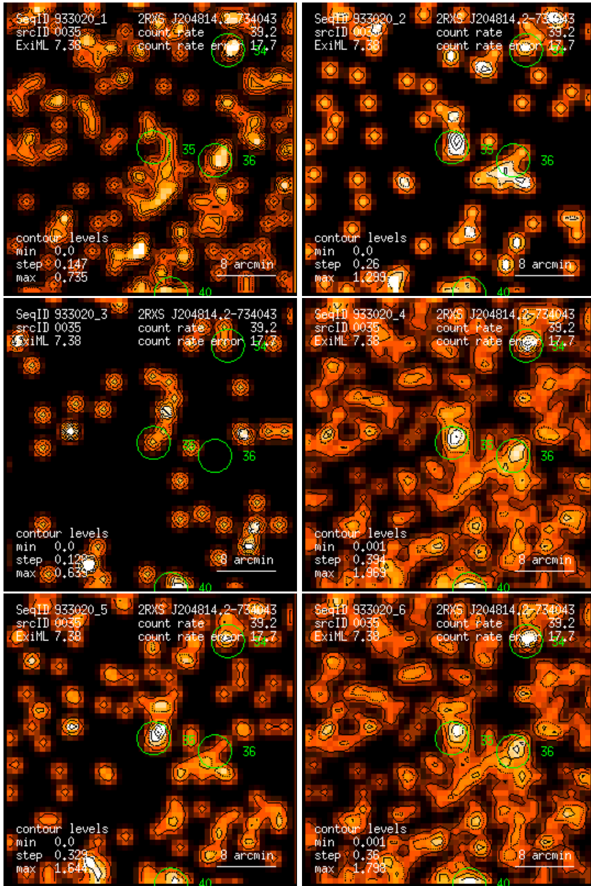
Figure 35: RASS 933020: detection 0035: band rate images, Gaussian filter: (1) PSPC channels 11 – 41, (2) 52 – 90, (3) 91 – 201, (4) 11 – 235, (5) 52 – 201, (6) 11 – 201. Broad band rates in counts/ks. Band rate contour levels in counts/ks/arcmin 2 .
