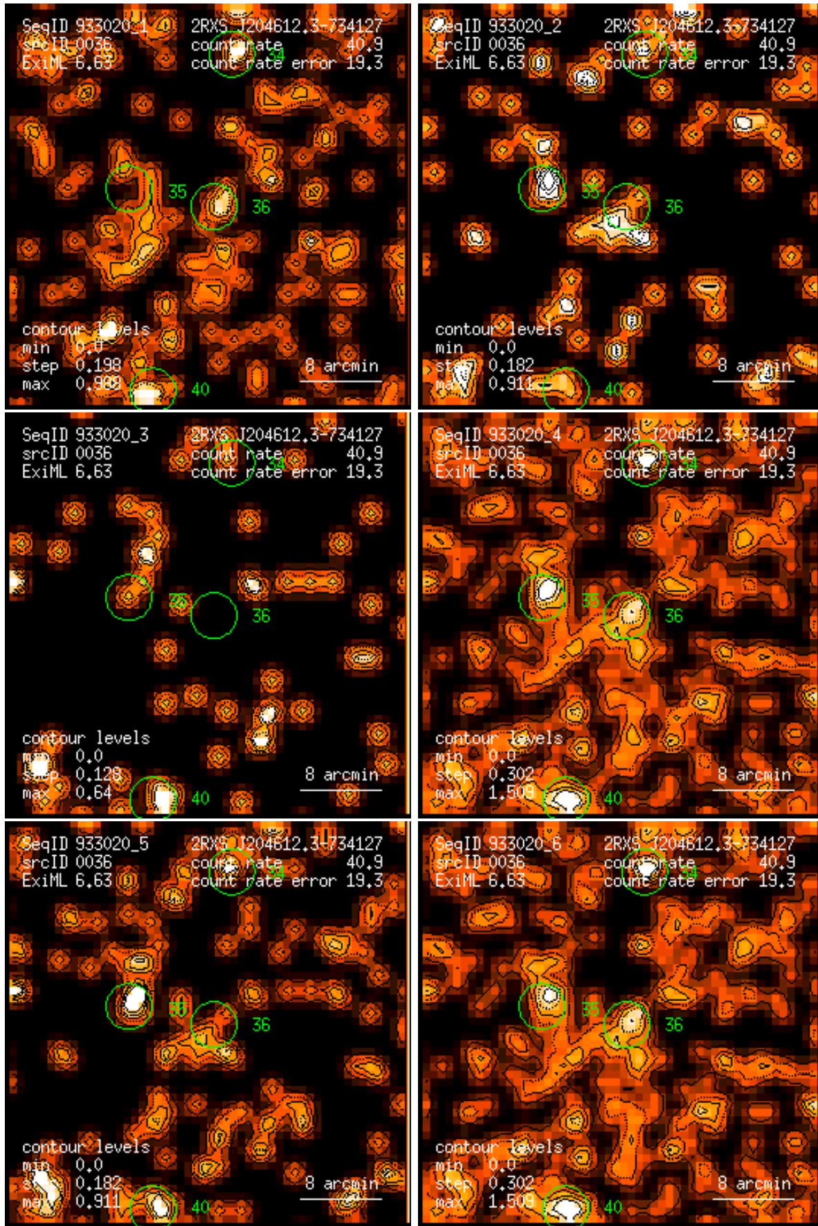
Figure 36: RASS 933020: detection 0036: band rate images, Gaussian filter: (1) PSPC channels 11 – 41, (2) 52 – 90, (3) 91 – 201, (4) 11 – 235, (5) 52 – 201, (6) 11 – 201. Broad band rates in counts/ks. Band rate contour levels in counts/ks/arcmin 2 .
