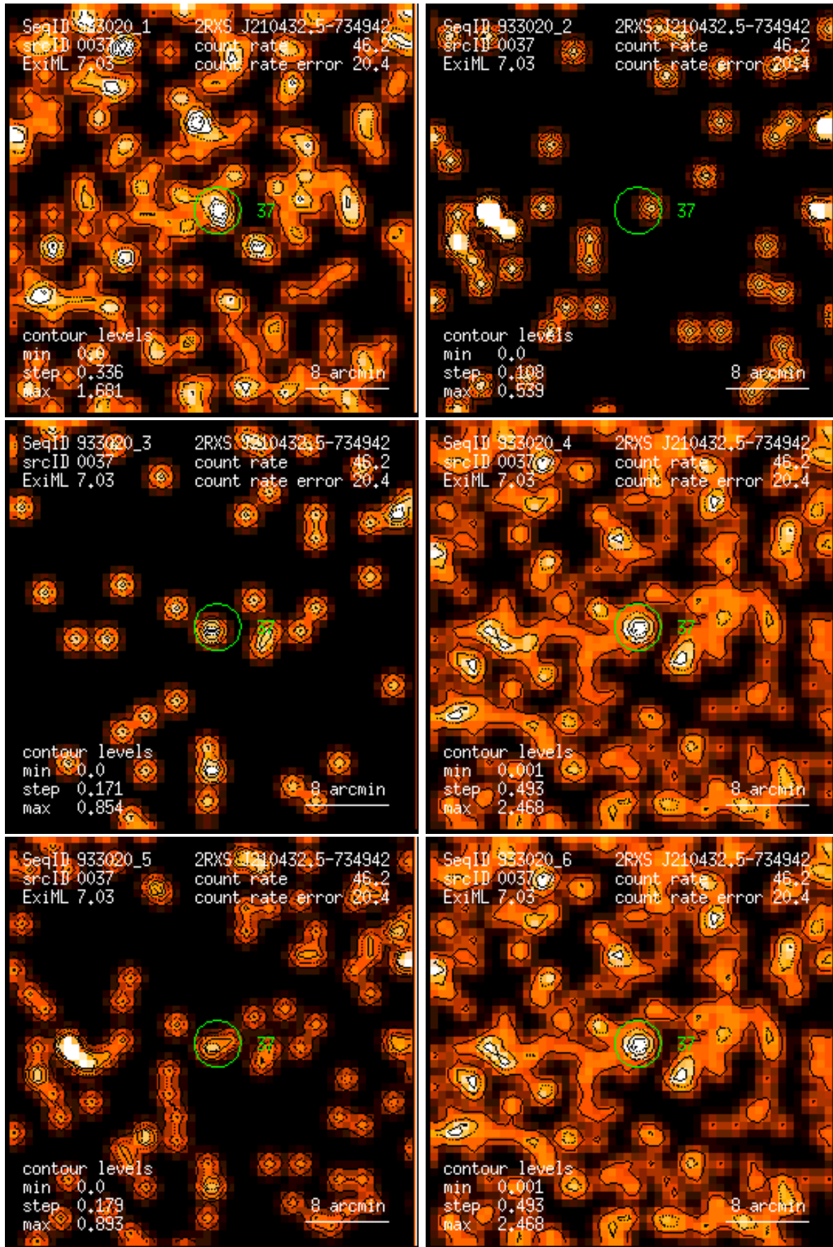
Figure 37: RASS 933020: detection 0037: band rate images, Gaussian filter: (1) PSPC channels 11 – 41, (2) 52 – 90, (3) 91 – 201, (4) 11 – 235, (5) 52 – 201, (6) 11 – 201. Broad band rates in counts/ks. Band rate contour levels in counts/ks/arcmin 2 .
