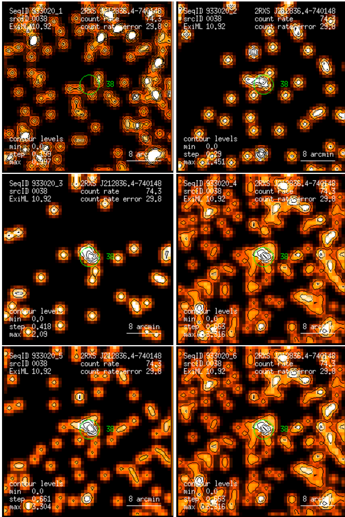
Figure 38: RASS 933020: detection 0038: band rate images, Gaussian filter: (1) PSPC channels 11 – 41, (2) 52 – 90, (3) 91 – 201, (4) 11 – 235, (5) 52 – 201, (6) 11 – 201. Broad band rates in counts/ks. Band rate contour levels in counts/ks/arcmin 2 .
