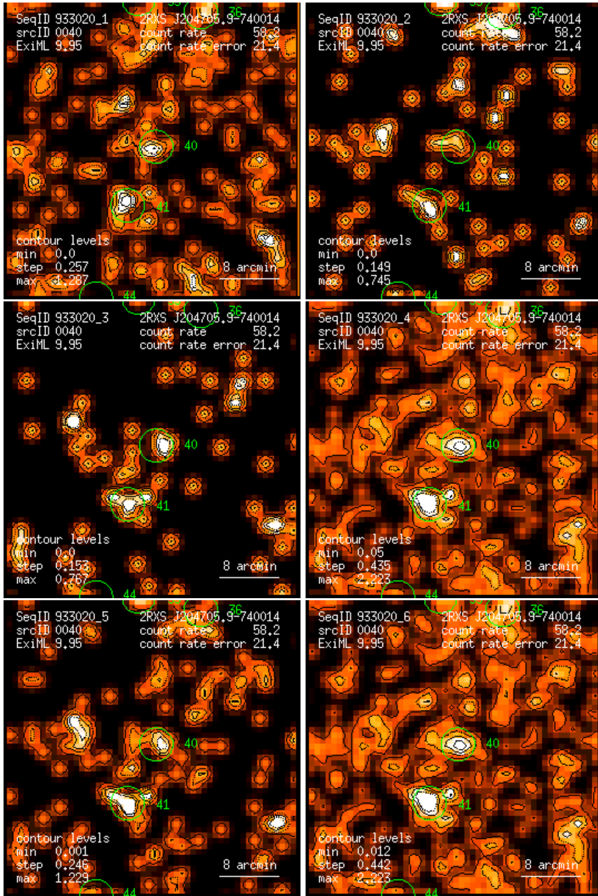
Figure 40: RASS 933020: detection 0040: band rate images, Gaussian filter: (1) PSPC channels 11 – 41, (2) 52 – 90, (3) 91 – 201, (4) 11 – 235, (5) 52 – 201, (6) 11 – 201. Broad band rates in counts/ks. Band rate contour levels in counts/ks/arcmin 2 .
