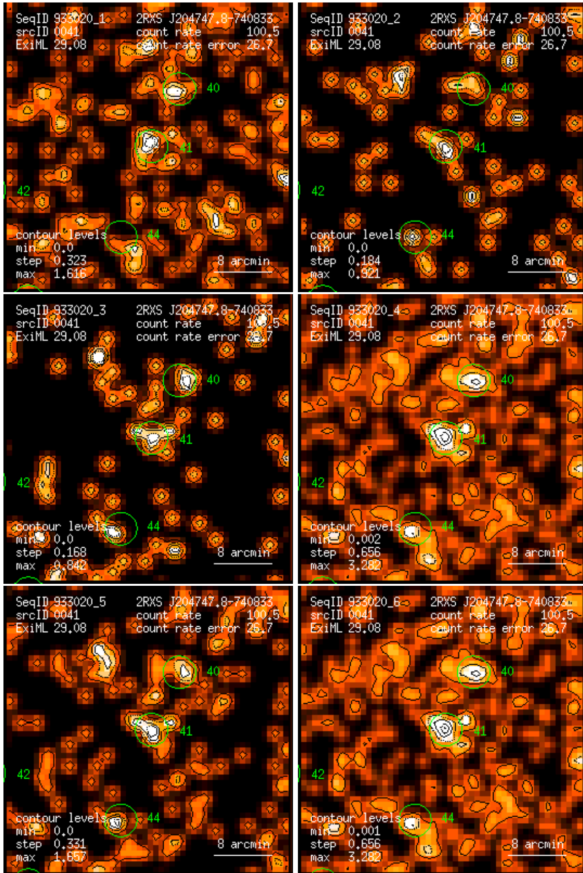
Figure 41: RASS 933020: detection 0041: band rate images, Gaussian filter: (1) PSPC channels 11 – 41, (2) 52 – 90, (3) 91 – 201, (4) 11 – 235, (5) 52 – 201, (6) 11 – 201. Broad band rates in counts/ks. Band rate contour levels in counts/ks/arcmin 2 .
