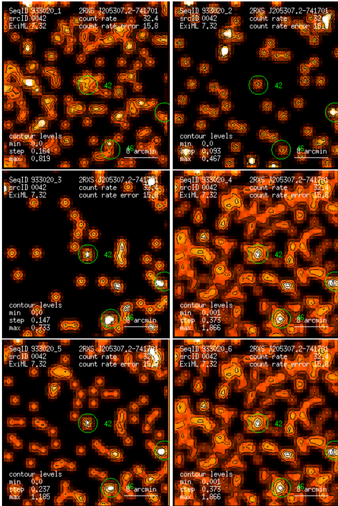
Figure 42: RASS 933020: detection 0042: band rate images, Gaussian filter: (1) PSPC channels 11 – 41, (2) 52 – 90, (3) 91 – 201, (4) 11 – 235, (5) 52 – 201, (6) 11 – 201. Broad band rates in counts/ks. Band rate contour levels in counts/ks/arcmin 2 .
