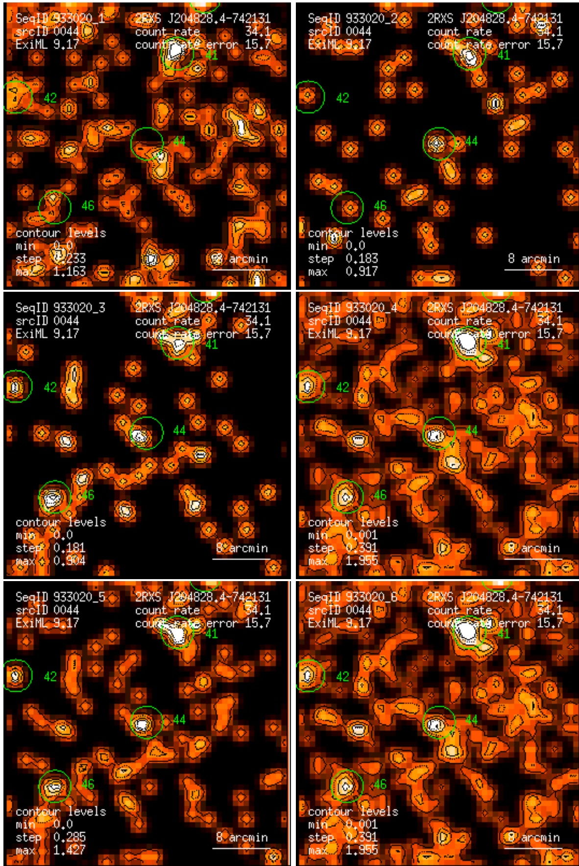
Figure 44: RASS 933020: detection 0044: band rate images, Gaussian filter: (1) PSPC channels 11 – 41, (2) 52 – 90, (3) 91 – 201, (4) 11 – 235, (5) 52 – 201, (6) 11 – 201. Broad band rates in counts/ks. Band rate contour levels in counts/ks/arcmin 2 .
