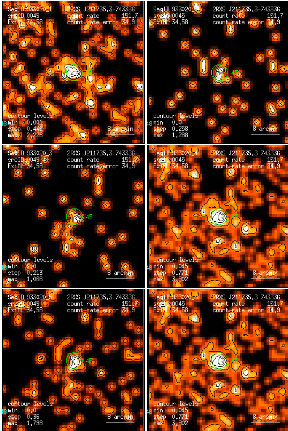
Figure 45: RASS 933020: detection 0045: band rate images, Gaussian filter: (1) PSPC channels 11 – 41, (2) 52 – 90, (3) 91 – 201, (4) 11 – 235, (5) 52 – 201, (6) 11 – 201. Broad band rates in counts/ks. Band rate contour levels in counts/ks/arcmin 2 .
