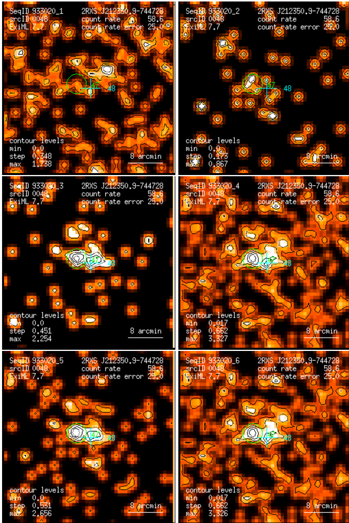
Figure 48: RASS 933020: detection 0048: band rate images, Gaussian filter: (1) PSPC channels 11 – 41, (2) 52 – 90, (3) 91 – 201, (4) 11 – 235, (5) 52 – 201, (6) 11 – 201. Broad band rates in counts/ks. Band rate contour levels in counts/ks/arcmin 2 .
