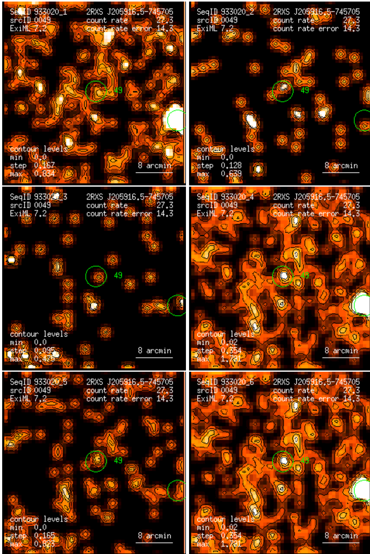
Figure 49: RASS 933020: detection 0049: band rate images, Gaussian filter: (1) PSPC channels 11 – 41, (2) 52 – 90, (3) 91 – 201, (4) 11 – 235, (5) 52 – 201, (6) 11 – 201. Broad band rates in counts/ks. Band rate contour levels in counts/ks/arcmin 2 .
