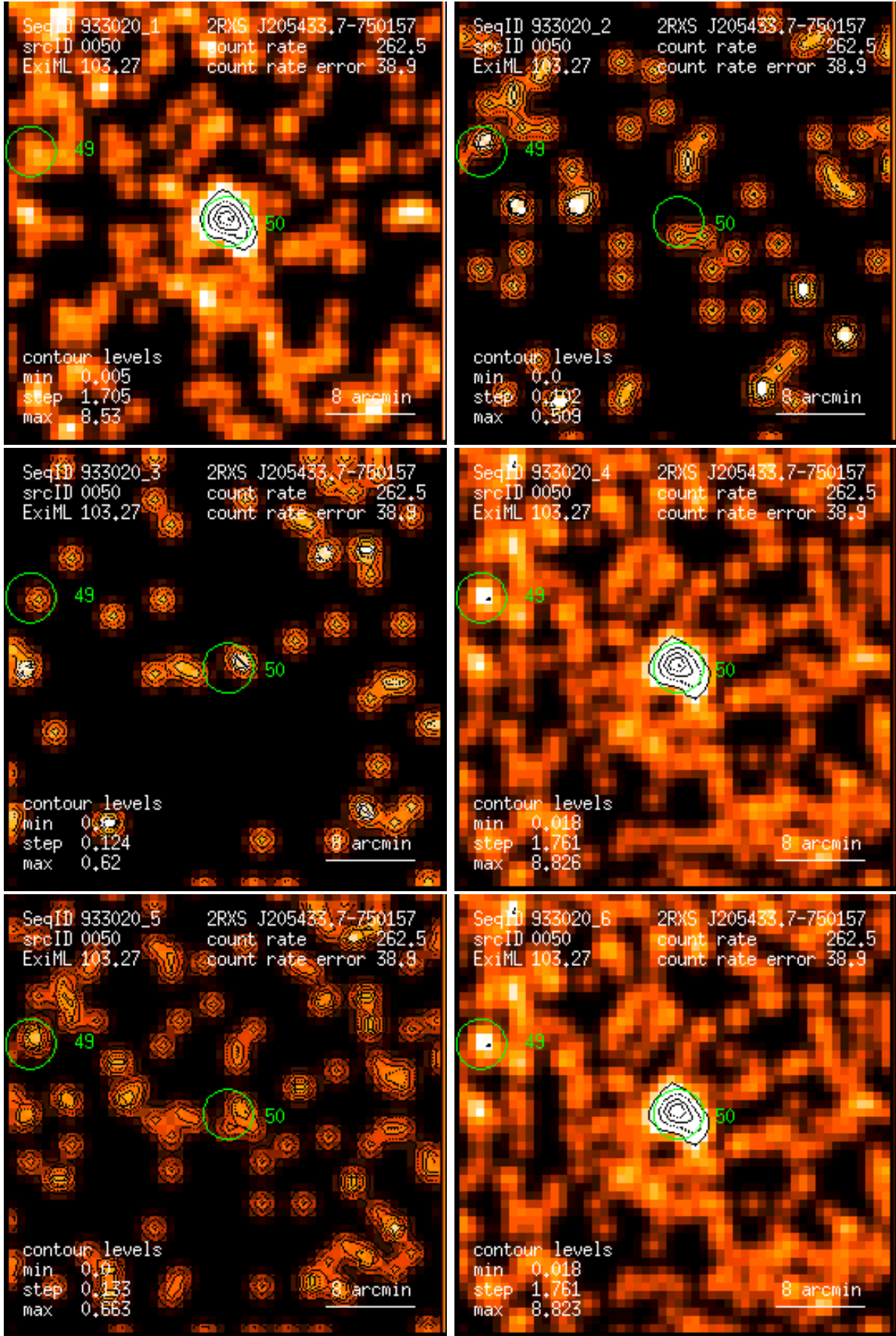
Figure 50: RASS 933020: detection 0050: band rate images, Gaussian filter: (1) PSPC channels 11 – 41, (2) 52 – 90, (3) 91 – 201, (4) 11 – 235, (5) 52 – 201, (6) 11 – 201. Broad band rates in counts/ks. Band rate contour levels in counts/ks/arcmin 2 .
