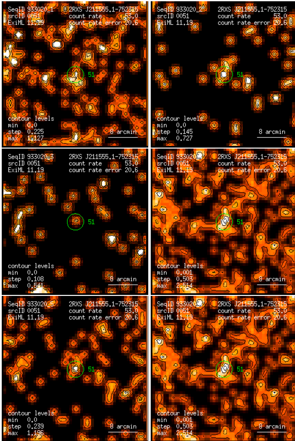
Figure 51: RASS 933020: detection 0051: band rate images, Gaussian filter: (1) PSPC channels 11 – 41, (2) 52 – 90, (3) 91 – 201, (4) 11 – 235, (5) 52 – 201, (6) 11 – 201. Broad band rates in counts/ks. Band rate contour levels in counts/ks/arcmin 2 .
