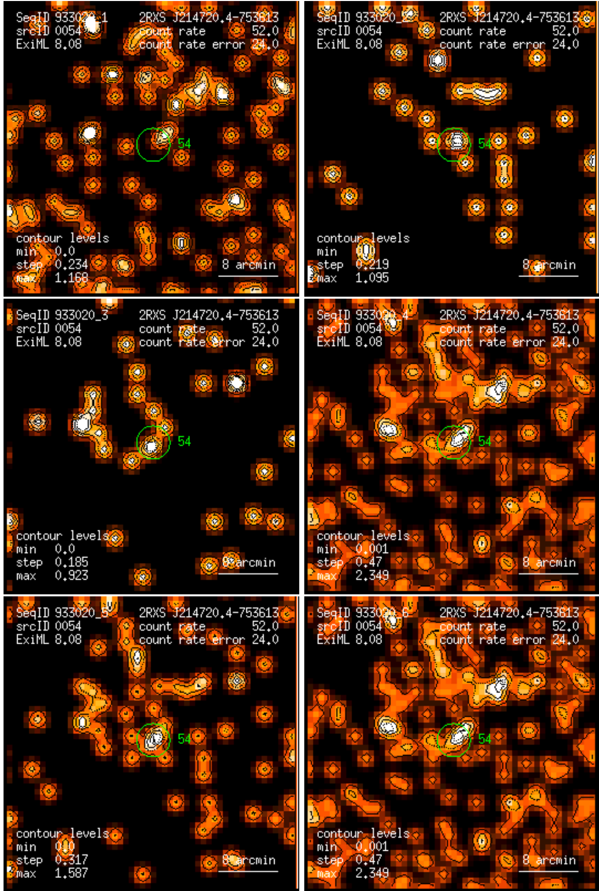
Figure 54: RASS 933020: detection 0054: band rate images, Gaussian filter: (1) PSPC channels 11 – 41, (2) 52 – 90, (3) 91 – 201, (4) 11 – 235, (5) 52 – 201, (6) 11 – 201. Broad band rates in counts/ks. Band rate contour levels in counts/ks/arcmin 2 .
