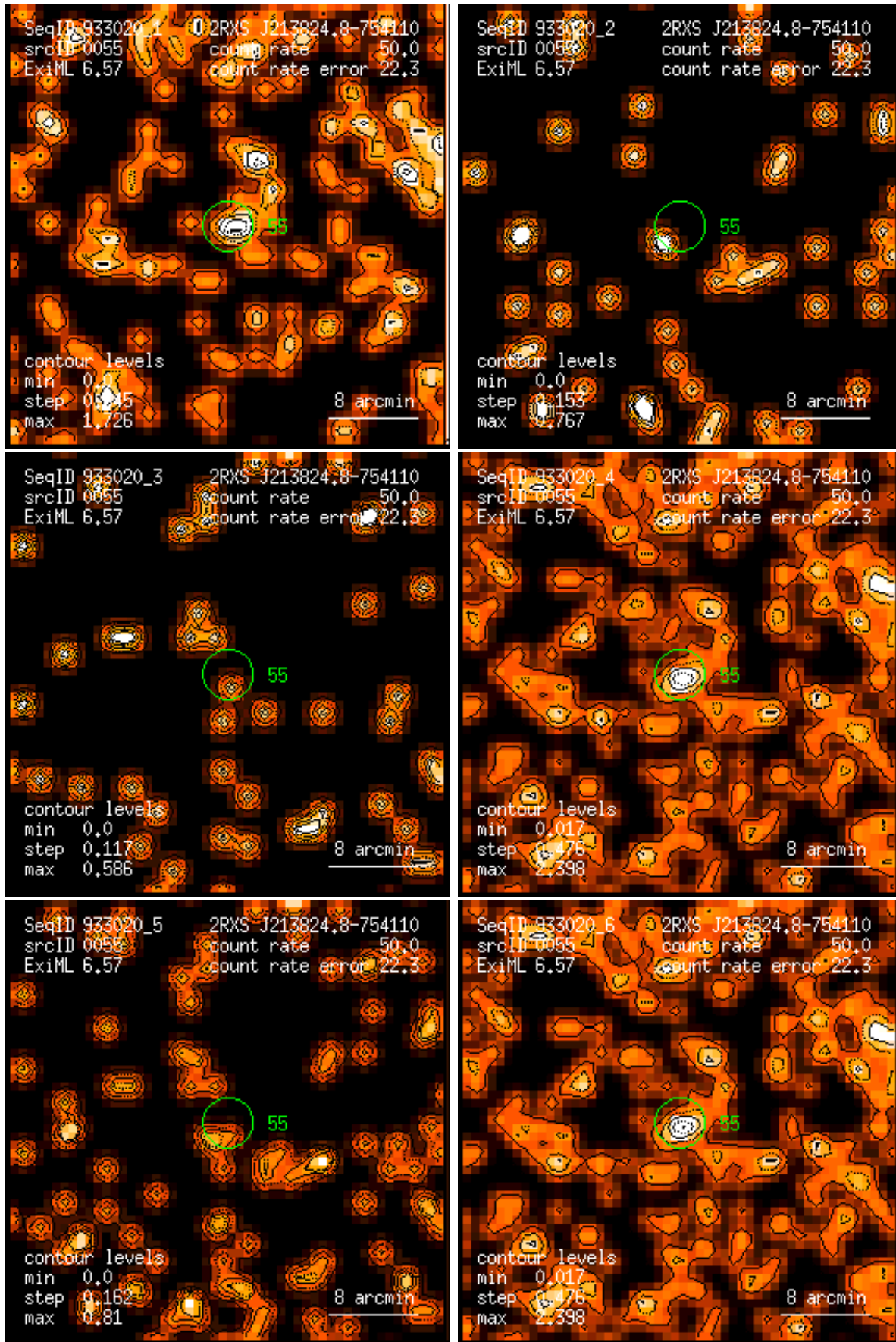
Figure 55: RASS 933020: detection 0055: band rate images, Gaussian filter: (1) PSPC channels 11 – 41, (2) 52 – 90, (3) 91 – 201, (4) 11 – 235, (5) 52 – 201, (6) 11 – 201. Broad band rates in counts/ks. Band rate contour levels in counts/ks/arcmin 2 .
