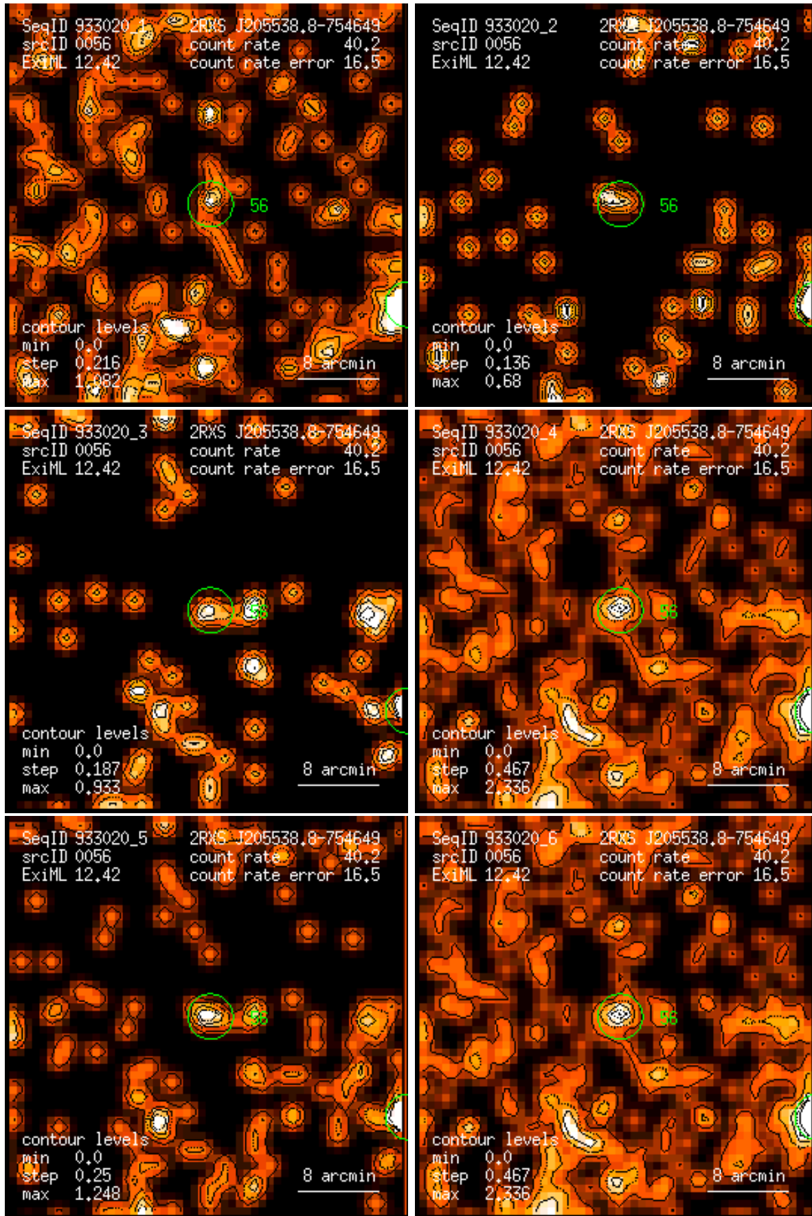
Figure 56: RASS 933020: detection 0056: band rate images, Gaussian filter: (1) PSPC channels 11 – 41, (2) 52 – 90, (3) 91 – 201, (4) 11 – 235, (5) 52 – 201, (6) 11 – 201. Broad band rates in counts/ks. Band rate contour levels in counts/ks/arcmin 2 .
