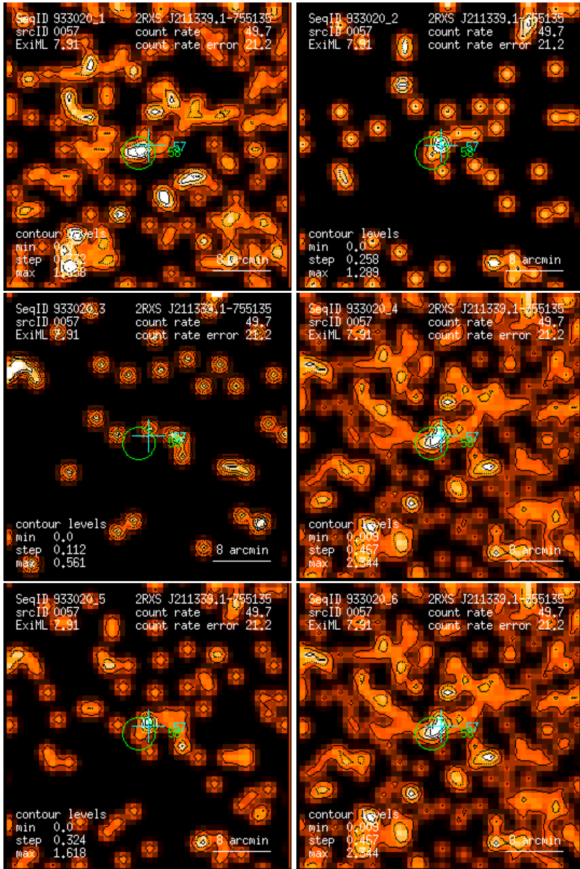
Figure 57: RASS 933020: detection 0057: band rate images, Gaussian filter: (1) PSPC channels 11 – 41, (2) 52 – 90, (3) 91 – 201, (4) 11 – 235, (5) 52 – 201, (6) 11 – 201. Broad band rates in counts/ks. Band rate contour levels in counts/ks/arcmin 2 .
