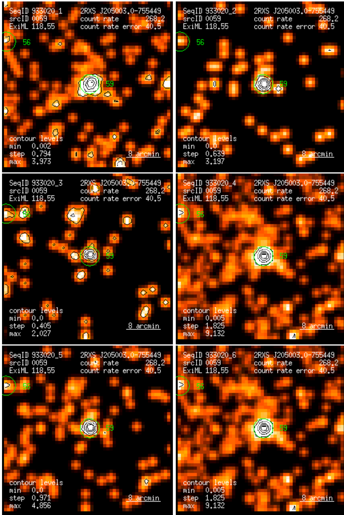
Figure 59: RASS 933020: detection 0059: band rate images, Gaussian filter: (1) PSPC channels 11 – 41, (2) 52 – 90, (3) 91 – 201, (4) 11 – 235, (5) 52 – 201, (6) 11 – 201. Broad band rates in counts/ks. Band rate contour levels in counts/ks/arcmin 2 .
