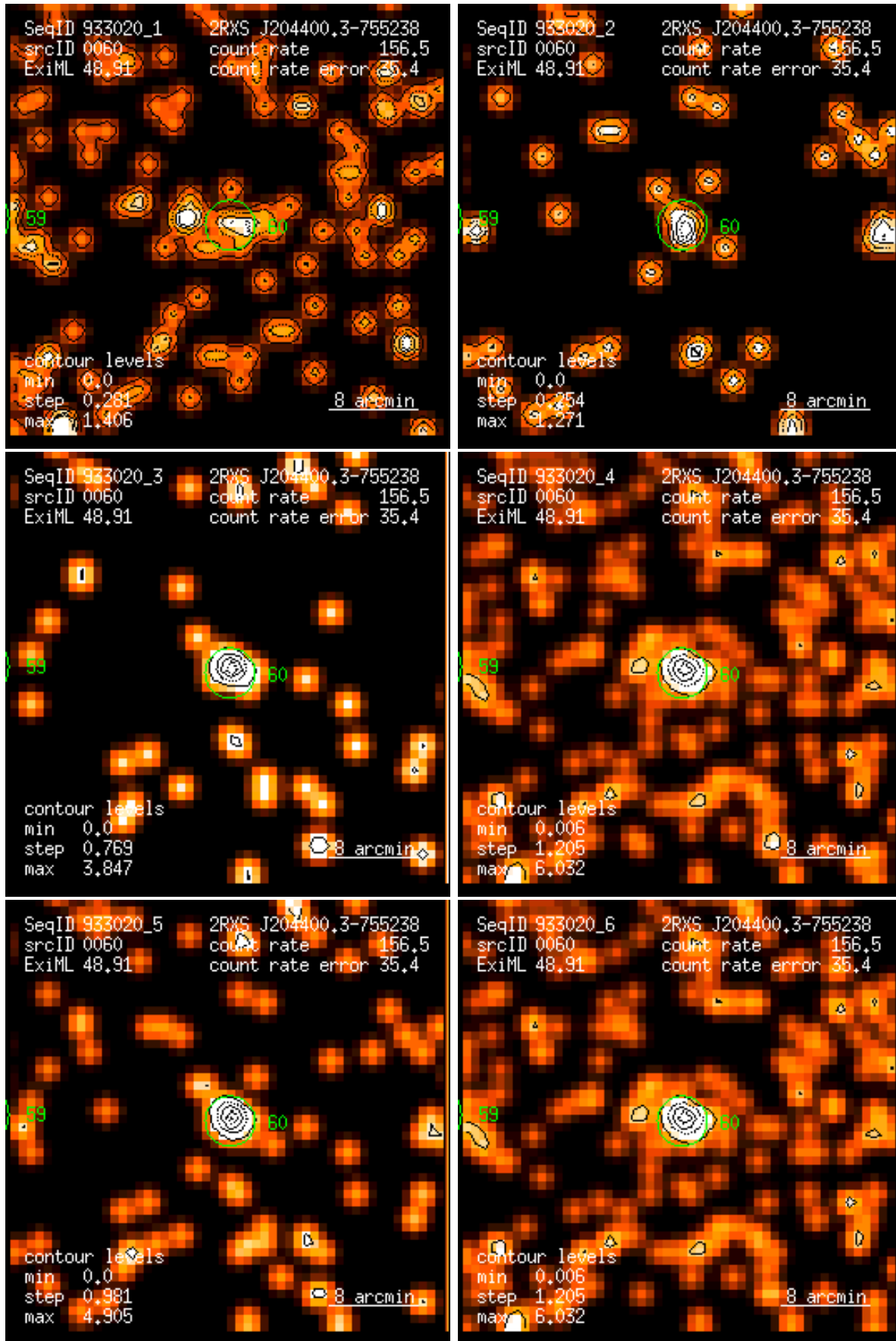
Figure 60: RASS 933020: detection 0060: band rate images, Gaussian filter: (1) PSPC channels 11 – 41, (2) 52 – 90, (3) 91 – 201, (4) 11 – 235, (5) 52 – 201, (6) 11 – 201. Broad band rates in counts/ks. Band rate contour levels in counts/ks/arcmin 2 .
