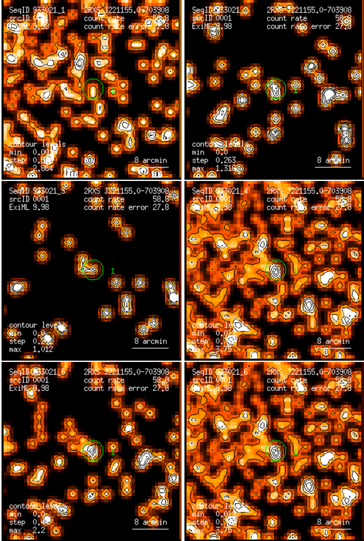
Figure 1: RASS 933021: detection 0001: band rate images, Gaussian filter: (1) PSPC channels 11 – 41, (2) 52 – 90, (3) 91 – 201, (4) 11 – 235, (5) 52 – 201, (6) 11 – 201. Broad band rates in counts/ks. Band rate contour levels in counts/ks/arcmin 2 .
