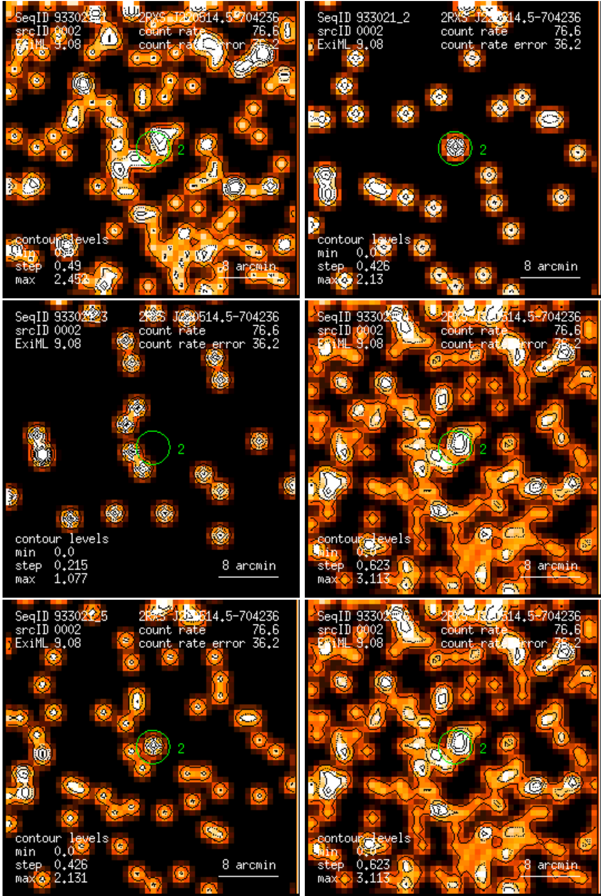
Figure 2: RASS 933021: detection 0002: band rate images, Gaussian filter: (1) PSPC channels 11 – 41, (2) 52 – 90, (3) 91 – 201, (4) 11 – 235, (5) 52 – 201, (6) 11 – 201. Broad band rates in counts/ks. Band rate contour levels in counts/ks/arcmin 2 .
