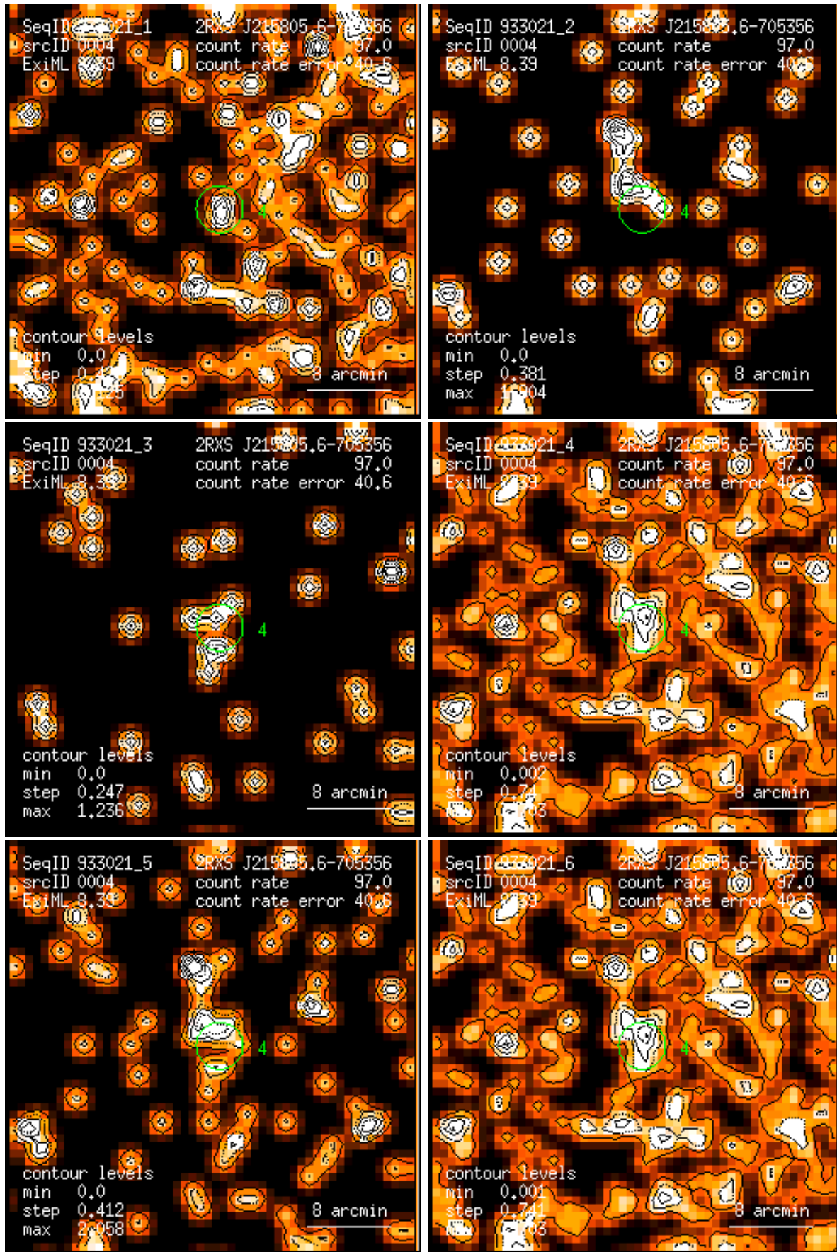
Figure 4: RASS 933021: detection 0004: band rate images, Gaussian filter: (1) PSPC channels 11 – 41, (2) 52 – 90, (3) 91 – 201, (4) 11 – 235, (5) 52 – 201, (6) 11 – 201. Broad band rates in counts/ks. Band rate contour levels in counts/ks/arcmin 2 .
