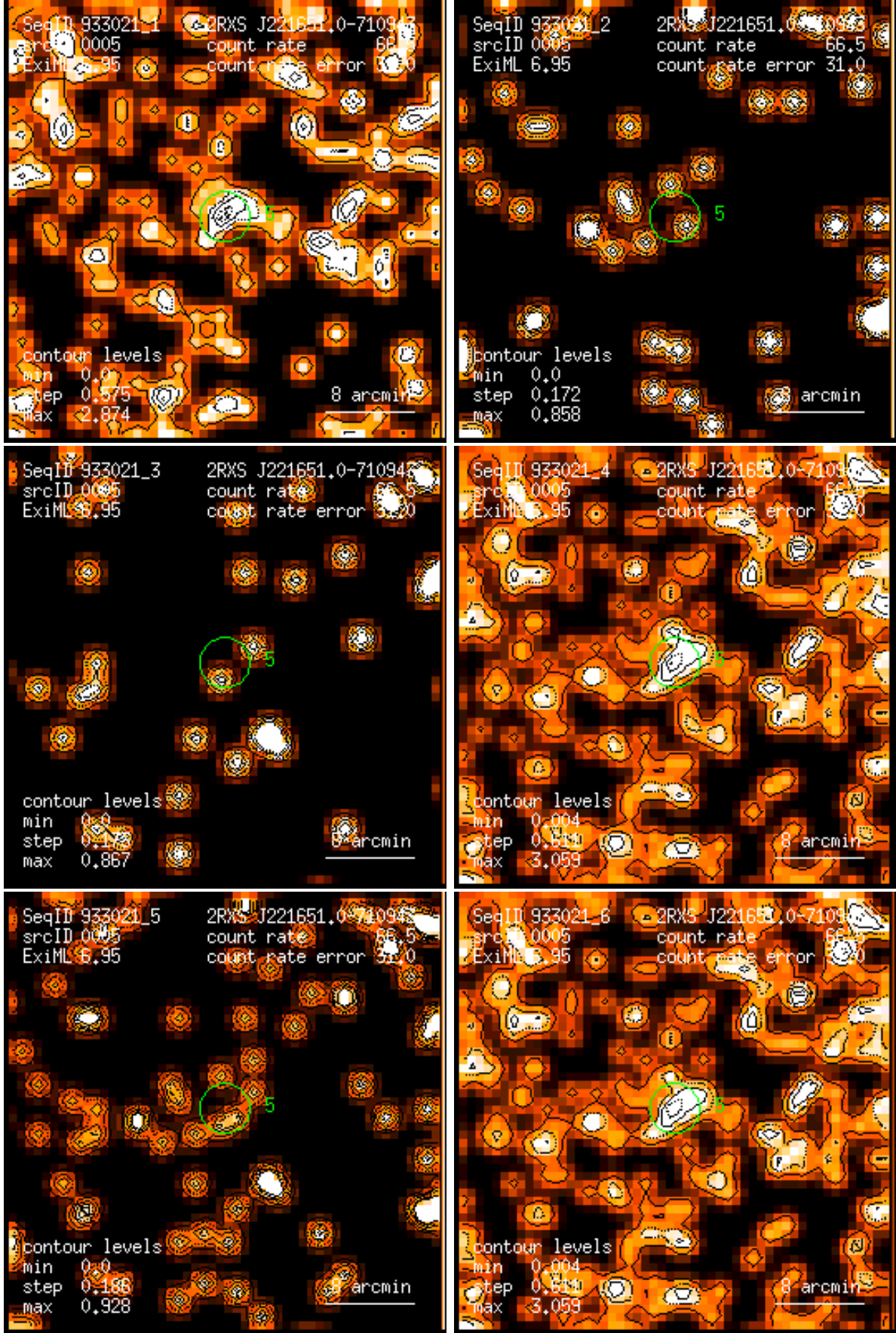
Figure 5: RASS 933021: detection 0005: band rate images, Gaussian filter: (1) PSPC channels 11 – 41, (2) 52 – 90, (3) 91 – 201, (4) 11 – 235, (5) 52 – 201, (6) 11 – 201. Broad band rates in counts/ks. Band rate contour levels in counts/ks/arcmin 2 .
