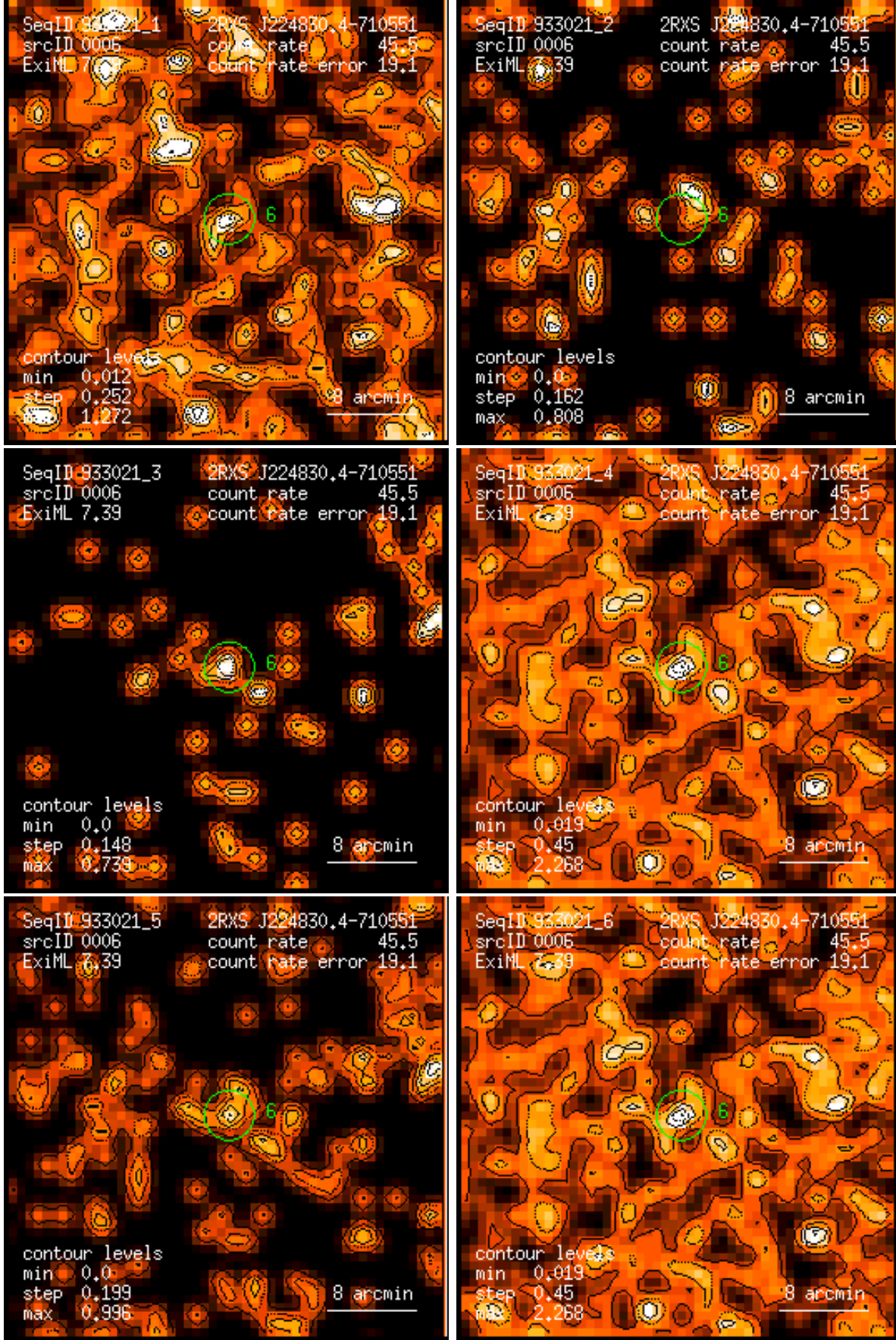
Figure 6: RASS 933021: detection 0006: band rate images, Gaussian filter: (1) PSPC channels 11 – 41, (2) 52 – 90, (3) 91 – 201, (4) 11 – 235, (5) 52 – 201, (6) 11 – 201. Broad band rates in counts/ks. Band rate contour levels in counts/ks/arcmin 2 .
