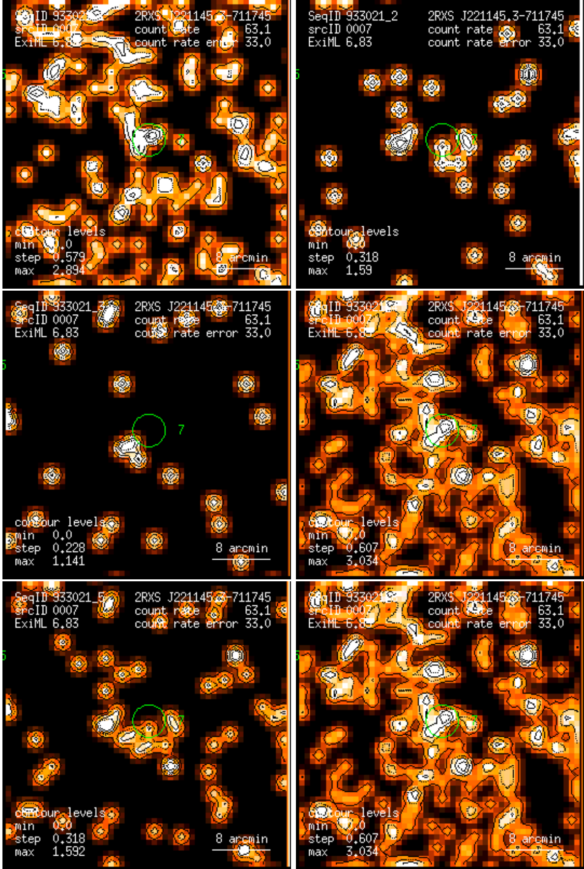
Figure 7: RASS 933021: detection 0007: band rate images, Gaussian filter: (1) PSPC channels 11 – 41, (2) 52 – 90, (3) 91 – 201, (4) 11 – 235, (5) 52 – 201, (6) 11 – 201. Broad band rates in counts/ks. Band rate contour levels in counts/ks/arcmin 2 .
