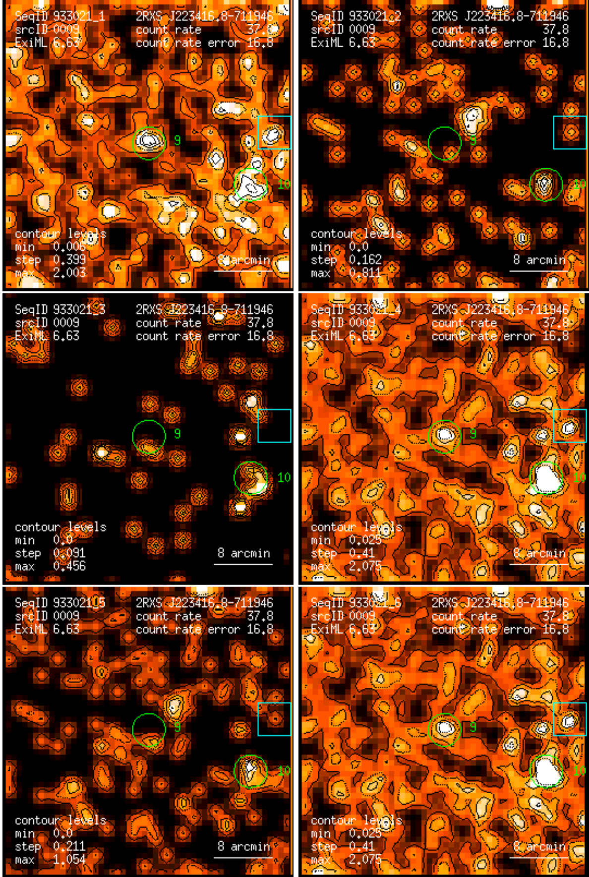
Figure 9: RASS 933021: detection 0009: band rate images, Gaussian filter: (1) PSPC channels 11 – 41, (2) 52 – 90, (3) 91 – 201, (4) 11 – 235, (5) 52 – 201, (6) 11 – 201. Broad band rates in counts/ks. Band rate contour levels in counts/ks/arcmin 2 .
