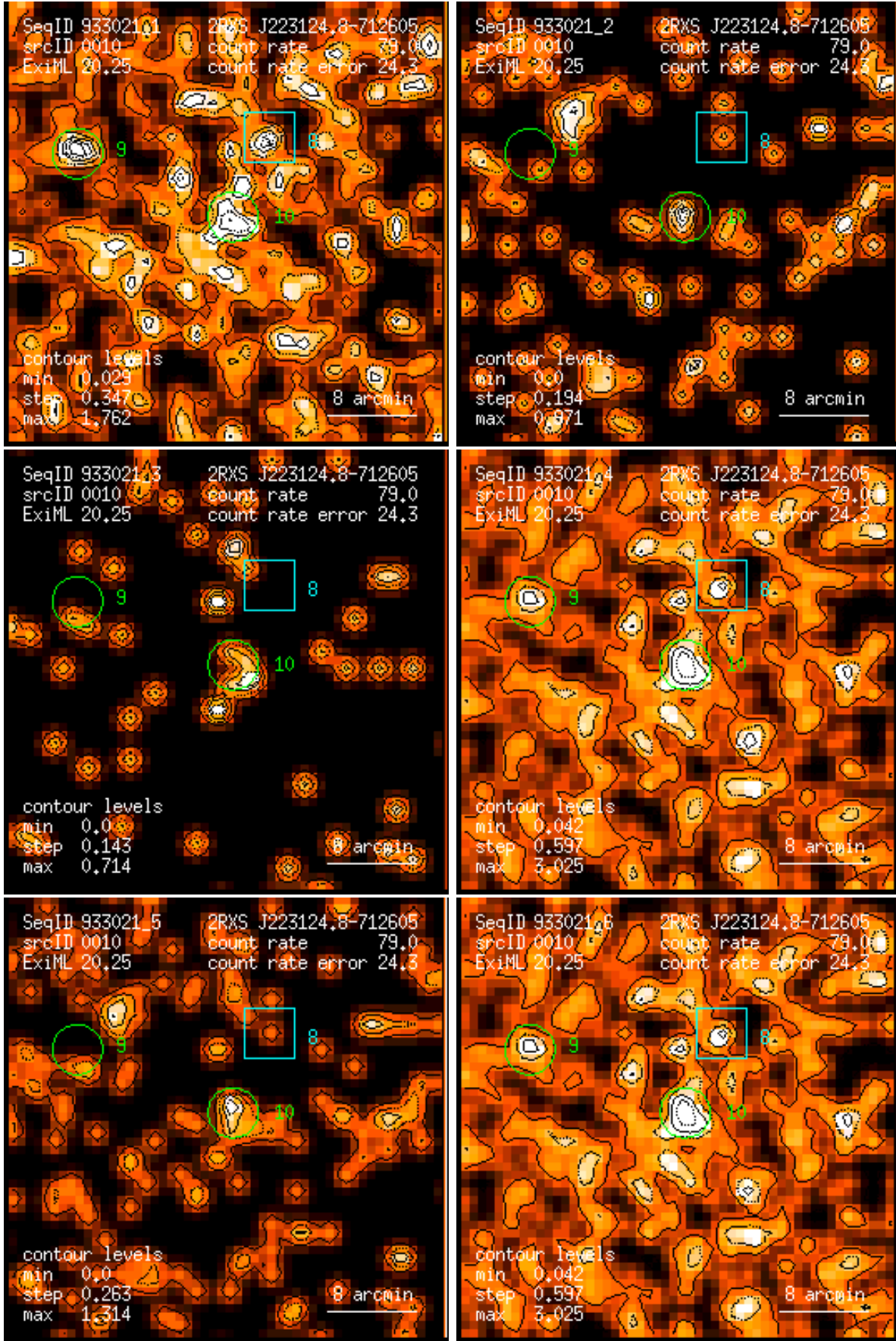
Figure 10: RASS 933021: detection 0010: band rate images, Gaussian filter: (1) PSPC channels 11 – 41, (2) 52 – 90, (3) 91 – 201, (4) 11 – 235, (5) 52 – 201, (6) 11 – 201. Broad band rates in counts/ks. Band rate contour levels in counts/ks/arcmin 2 .
