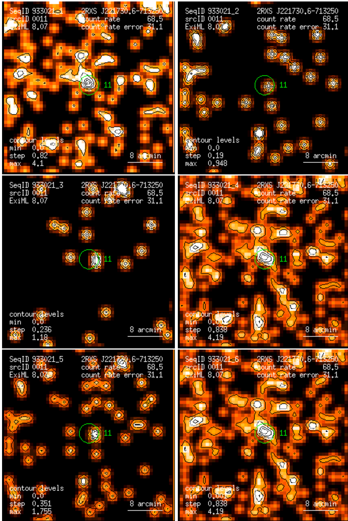
Figure 11: RASS 933021: detection 0011: band rate images, Gaussian filter: (1) PSPC channels 11 – 41, (2) 52 – 90, (3) 91 – 201, (4) 11 – 235, (5) 52 – 201, (6) 11 – 201. Broad band rates in counts/ks. Band rate contour levels in counts/ks/arcmin 2 .
