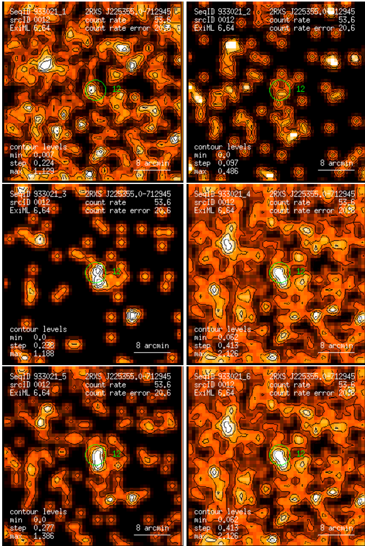
Figure 12: RASS 933021: detection 0012: band rate images, Gaussian filter: (1) PSPC channels 11 – 41, (2) 52 – 90, (3) 91 – 201, (4) 11 – 235, (5) 52 – 201, (6) 11 – 201. Broad band rates in counts/ks. Band rate contour levels in counts/ks/arcmin 2 .
