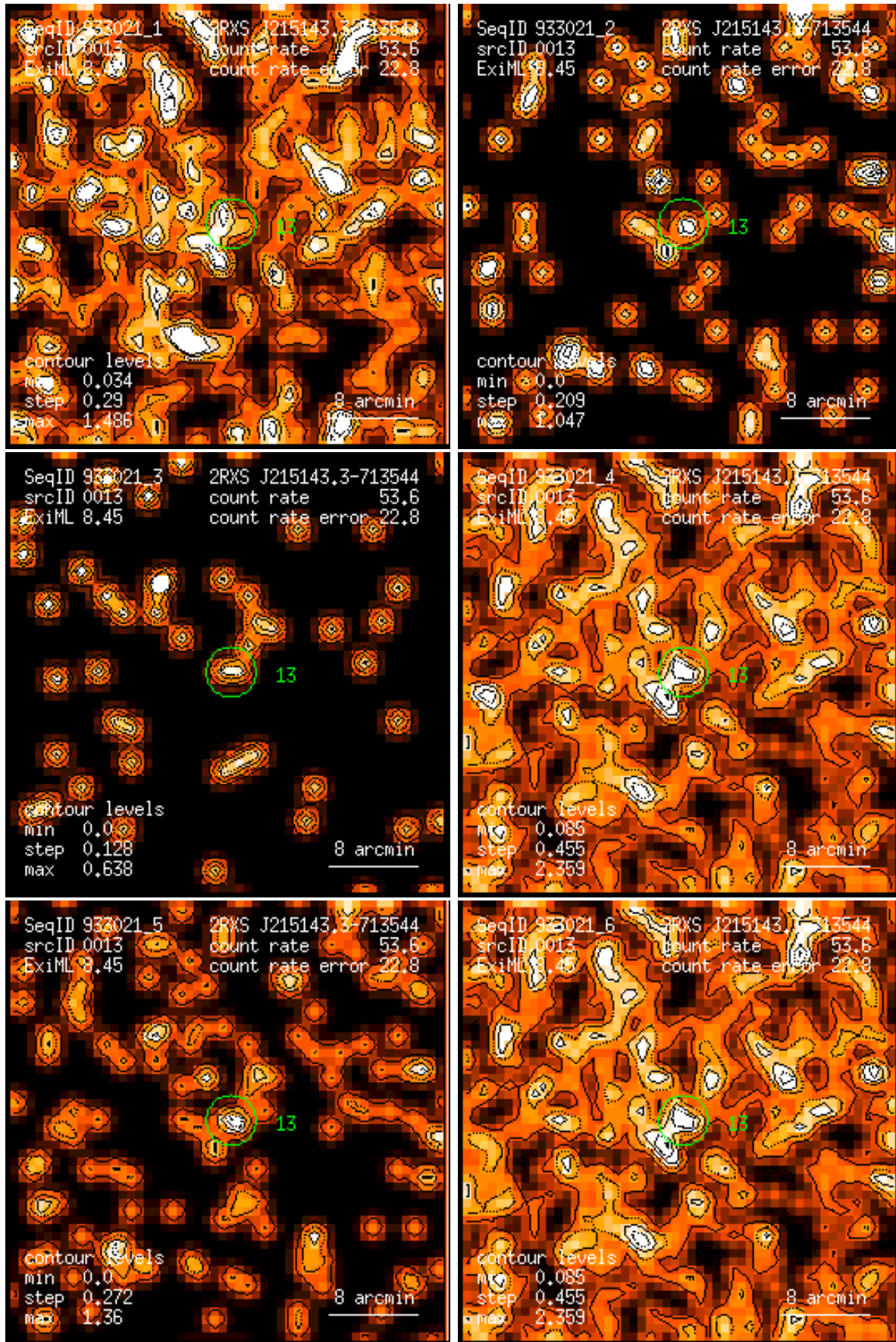
Figure 13: RASS 933021: detection 0013: band rate images, Gaussian filter: (1) PSPC channels 11 – 41, (2) 52 – 90, (3) 91 – 201, (4) 11 – 235, (5) 52 – 201, (6) 11 – 201. Broad band rates in counts/ks. Band rate contour levels in counts/ks/arcmin 2 .
