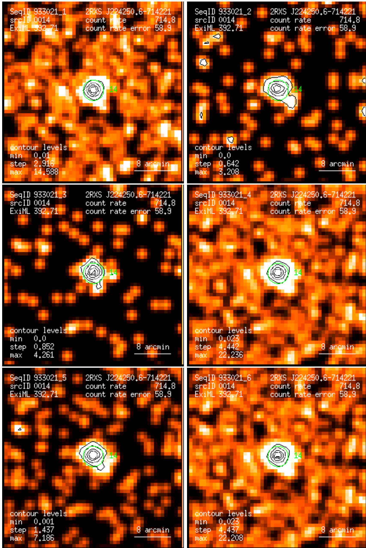
Figure 14: RASS 933021: detection 0014: band rate images, Gaussian filter: (1) PSPC channels 11 – 41, (2) 52 – 90, (3) 91 – 201, (4) 11 – 235, (5) 52 – 201, (6) 11 – 201. Broad band rates in counts/ks. Band rate contour levels in counts/ks/arcmin 2 .
