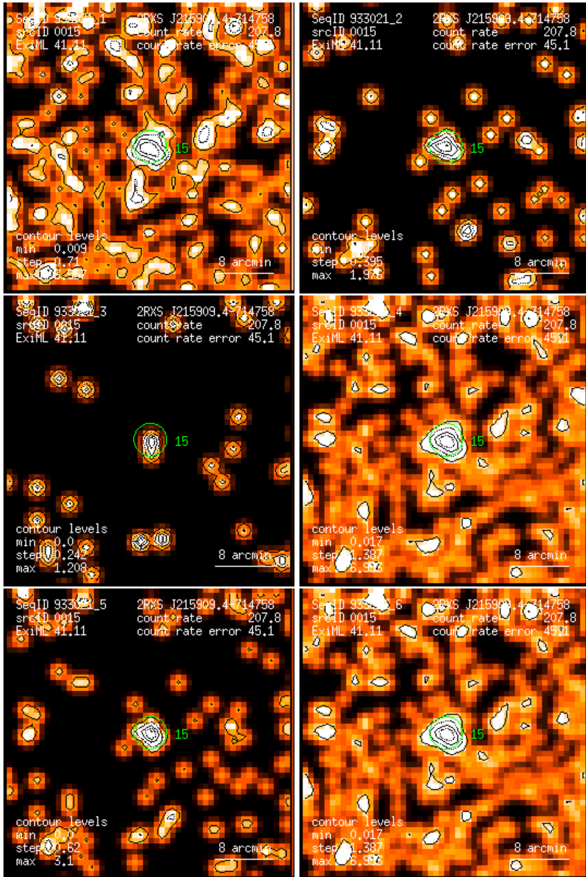
Figure 15: RASS 933021: detection 0015: band rate images, Gaussian filter: (1) PSPC channels 11 – 41, (2) 52 – 90, (3) 91 – 201, (4) 11 – 235, (5) 52 – 201, (6) 11 – 201. Broad band rates in counts/ks. Band rate contour levels in counts/ks/arcmin 2 .
