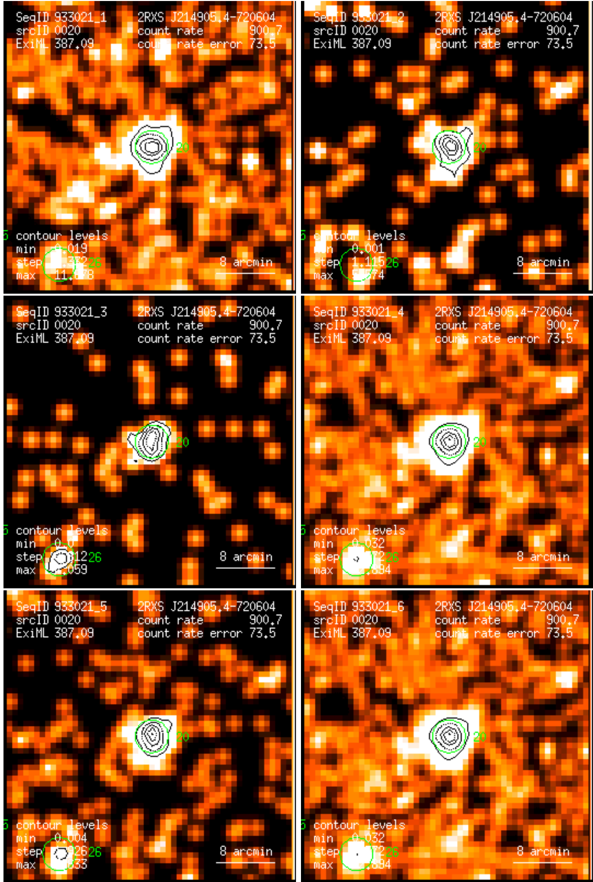
Figure 20: RASS 933021: detection 0020: band rate images, Gaussian filter: (1) PSPC channels 11 – 41, (2) 52 – 90, (3) 91 – 201, (4) 11 – 235, (5) 52 – 201, (6) 11 – 201. Broad band rates in counts/ks. Band rate contour levels in counts/ks/arcmin 2 .
