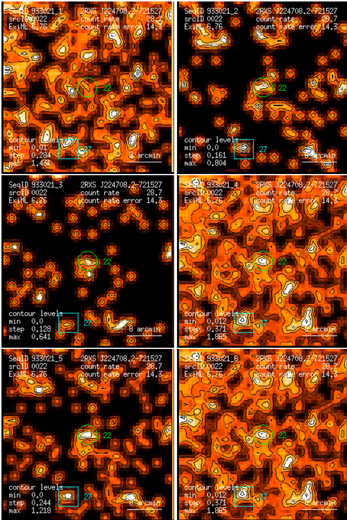
Figure 22: RASS 933021: detection 0022: band rate images, Gaussian filter: (1) PSPC channels 11 – 41, (2) 52 – 90, (3) 91 – 201, (4) 11 – 235, (5) 52 – 201, (6) 11 – 201. Broad band rates in counts/ks. Band rate contour levels in counts/ks/arcmin 2 .
