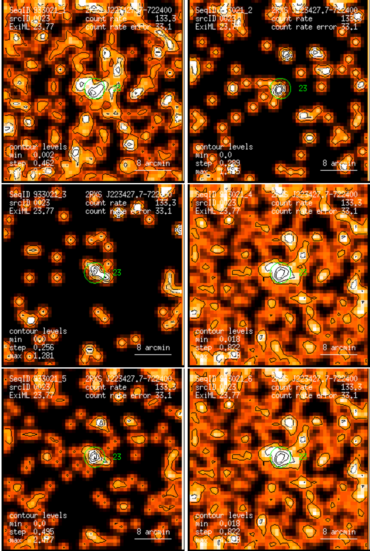
Figure 23: RASS 933021: detection 0023: band rate images, Gaussian filter: (1) PSPC channels 11 – 41, (2) 52 – 90, (3) 91 – 201, (4) 11 – 235, (5) 52 – 201, (6) 11 – 201. Broad band rates in counts/ks. Band rate contour levels in counts/ks/arcmin 2 .
