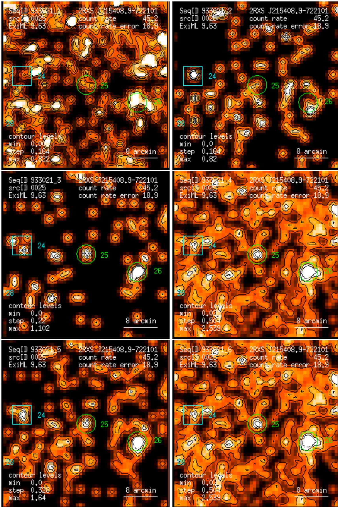
Figure 25: RASS 933021: detection 0025: band rate images, Gaussian filter: (1) PSPC channels 11 – 41, (2) 52 – 90, (3) 91 – 201, (4) 11 – 235, (5) 52 – 201, (6) 11 – 201. Broad band rates in counts/ks. Band rate contour levels in counts/ks/arcmin 2 .
