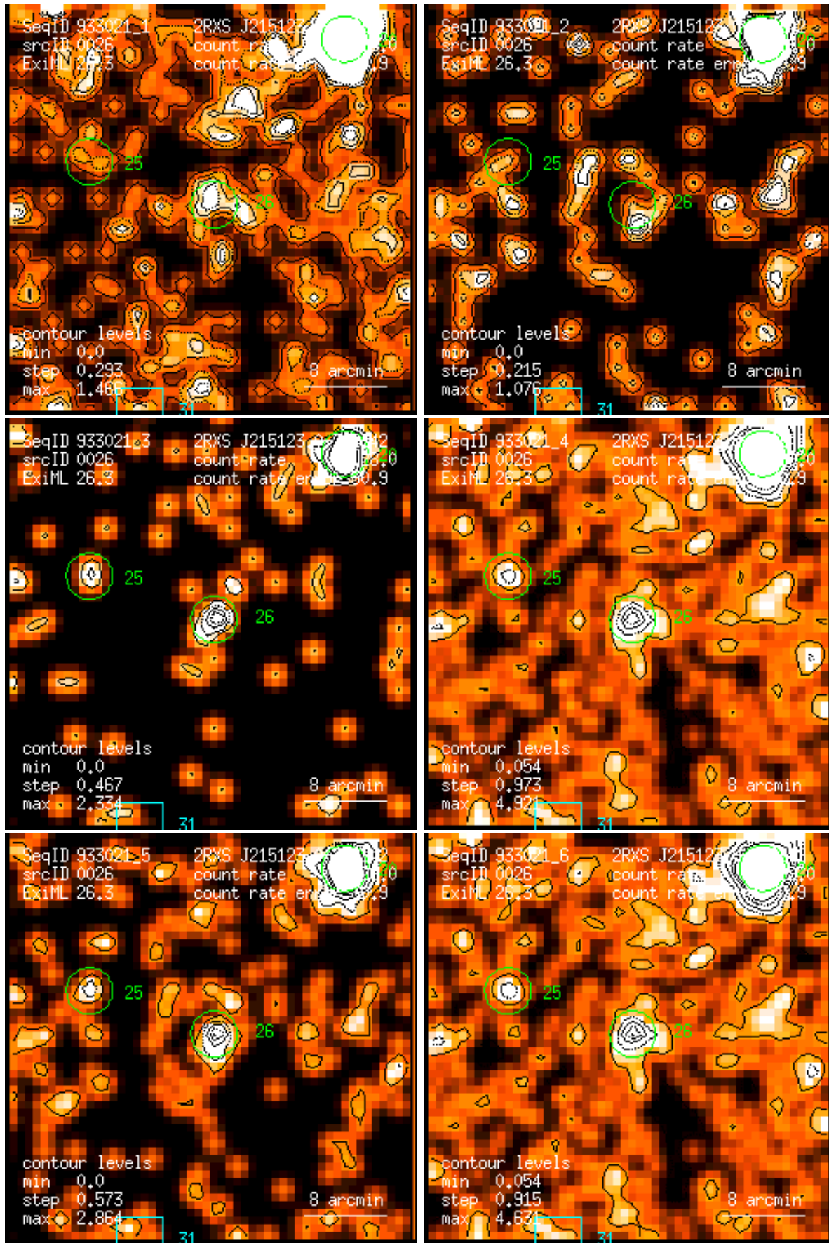
Figure 26: RASS 933021: detection 0026: band rate images, Gaussian filter: (1) PSPC channels 11 – 41, (2) 52 – 90, (3) 91 – 201, (4) 11 – 235, (5) 52 – 201, (6) 11 – 201. Broad band rates in counts/ks. Band rate contour levels in counts/ks/arcmin 2 .
